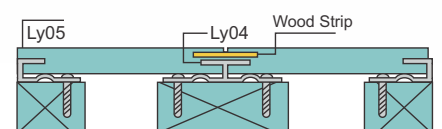
Cross-section Structure
